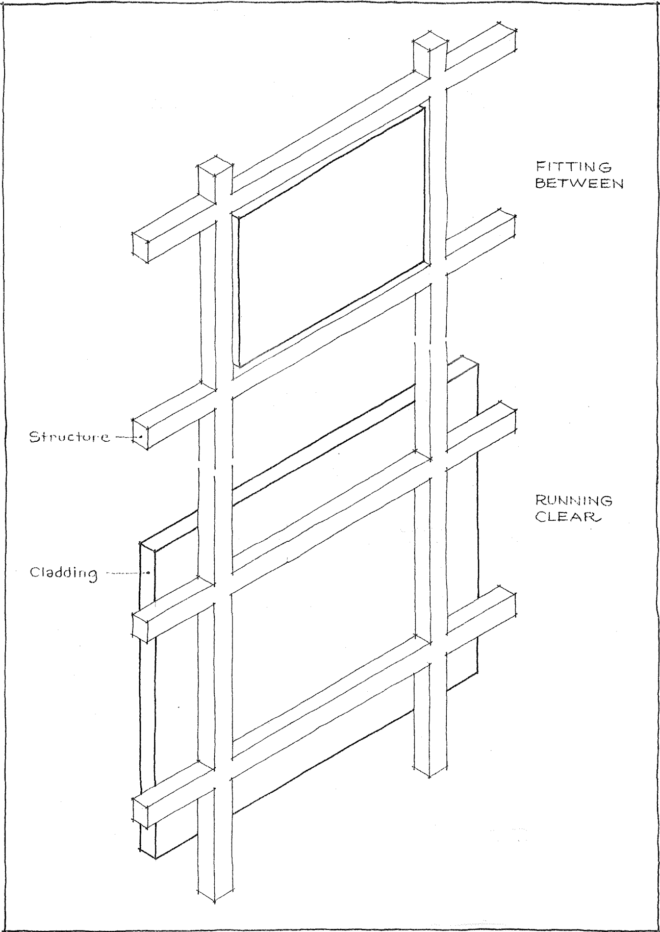
Structure to cladding joints
